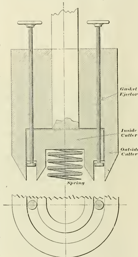
Railway & Locomotive Engineering MILLER'S GASKET CUTTER.
